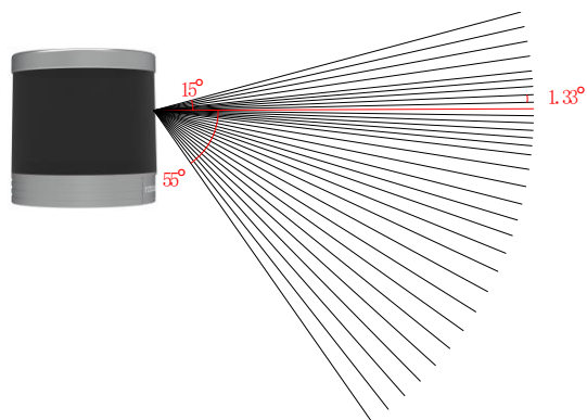
(b) Vertical Angular Distribution
