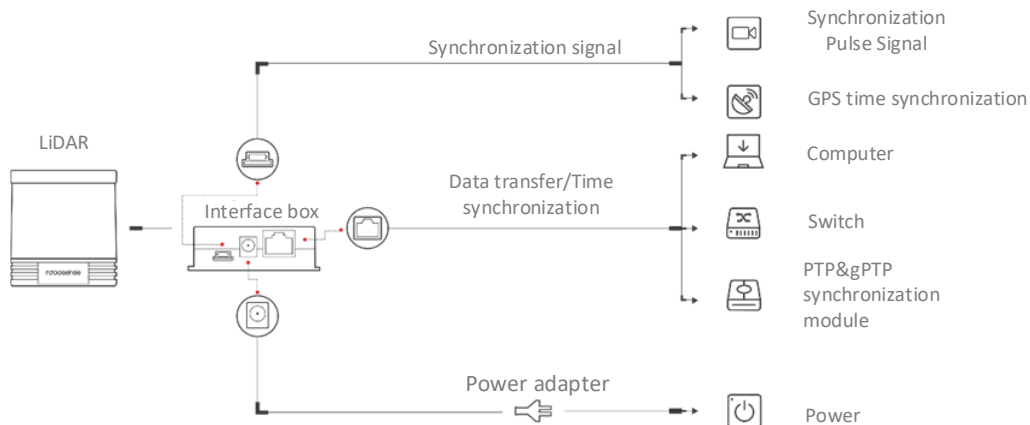
Figure 13 Interface Box Connection Diagram
