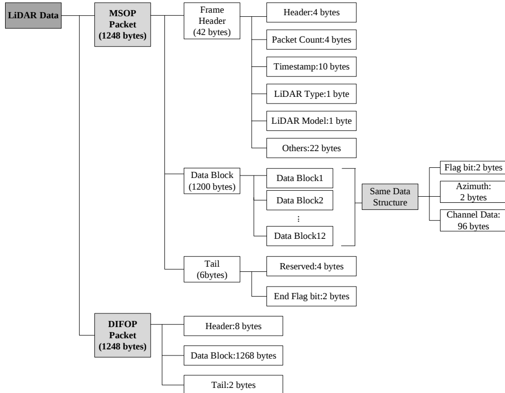
Figure 16 LiDAR Data Structure Illustration
