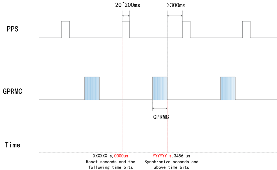
Figure 7 GPS Time Synchronization Timing Diagram
