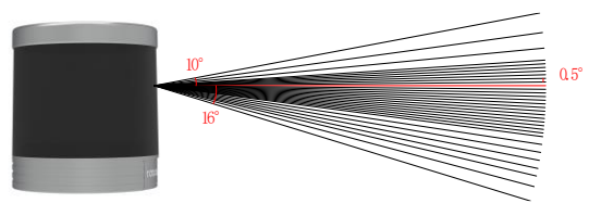
(b) Vertical Angular Distribution
