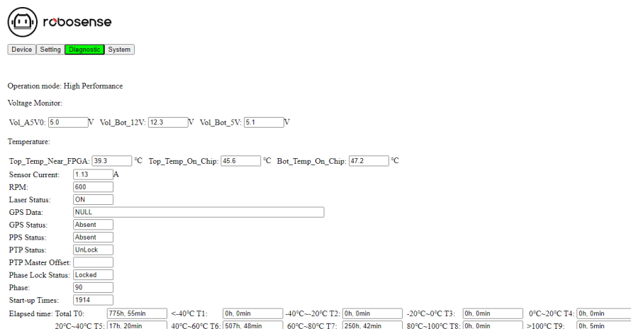
Figure 21 Web Interface Operating Status / Diagnostics
