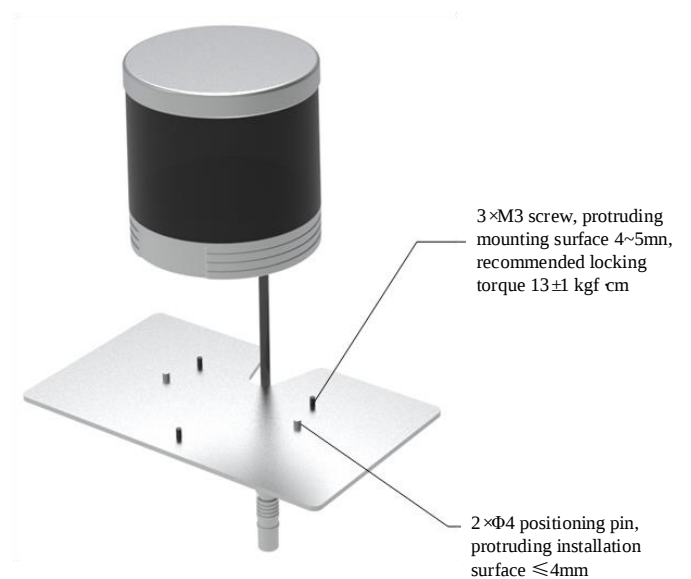
Figure 8 LiDAR Structural Installation Diagram
