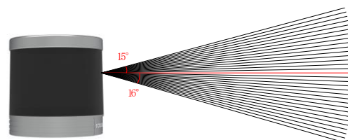
(b) Vertical Angular Distribution
