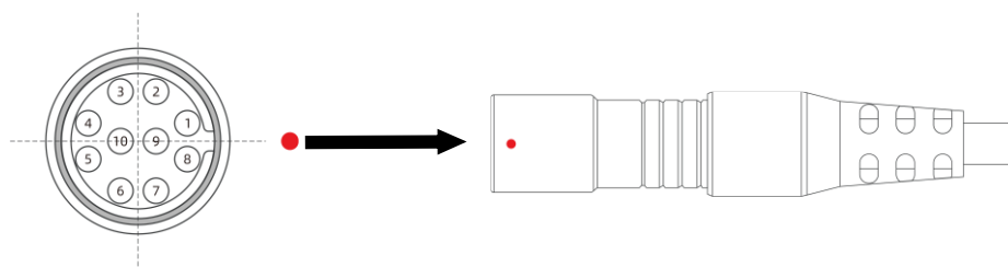
Figure 10 Pin Numbers of the Aviation Plug Interface
