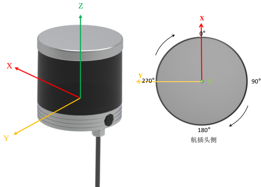
Figure 15 LiDAR Coordinate and Rotation Direction Illustration
