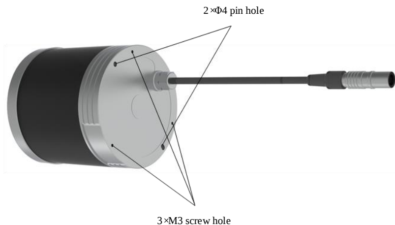
Figure 9 LiDAR Bottom Locator Pin and Screw Diagram
