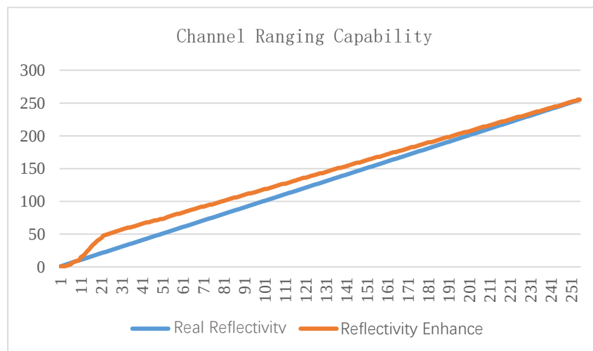
Figure 26 Reflectivity Mapping Chart
