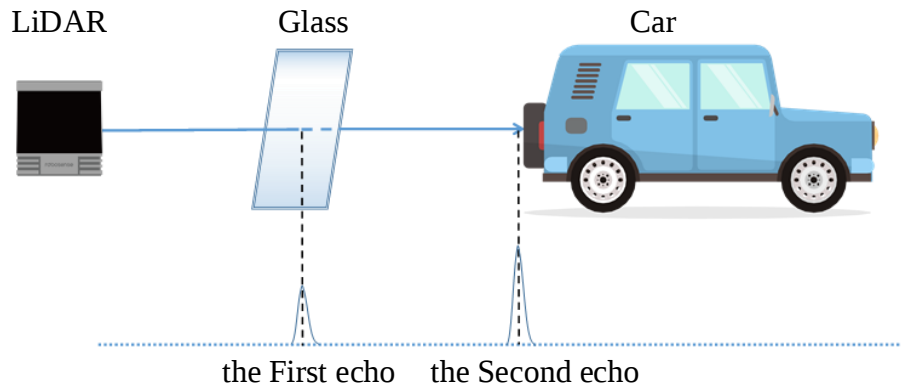
Figure 5 Dual Return Detection
